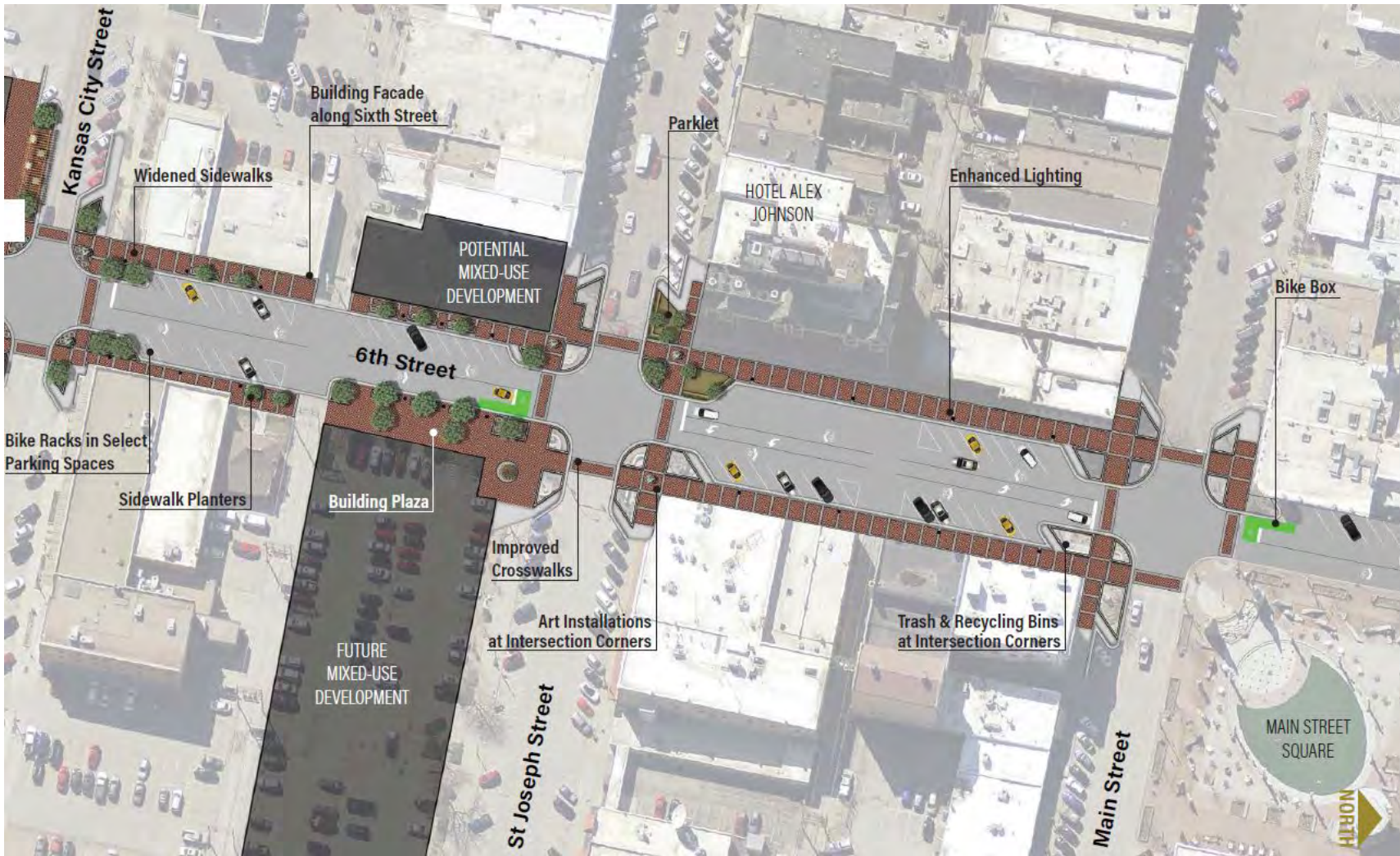
Figure 6. Corridor Concept, Kansas City Street to Main Street
